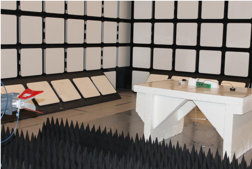
Photograph 1. Radiated emissions above 1000 MHz
