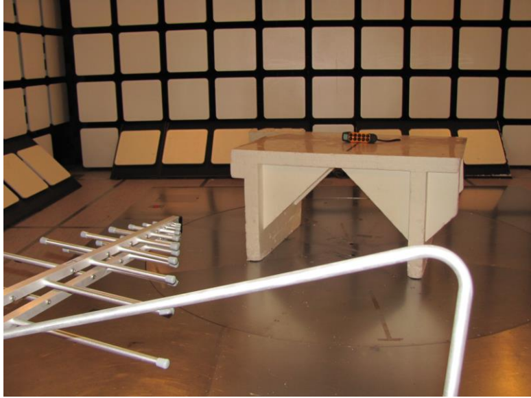
Photograph 1. Radiated emissions 30 - 1000 MHz
