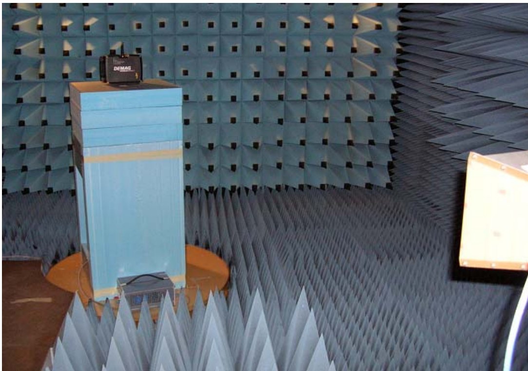
Radiated spurious emission 1-26 GHz
