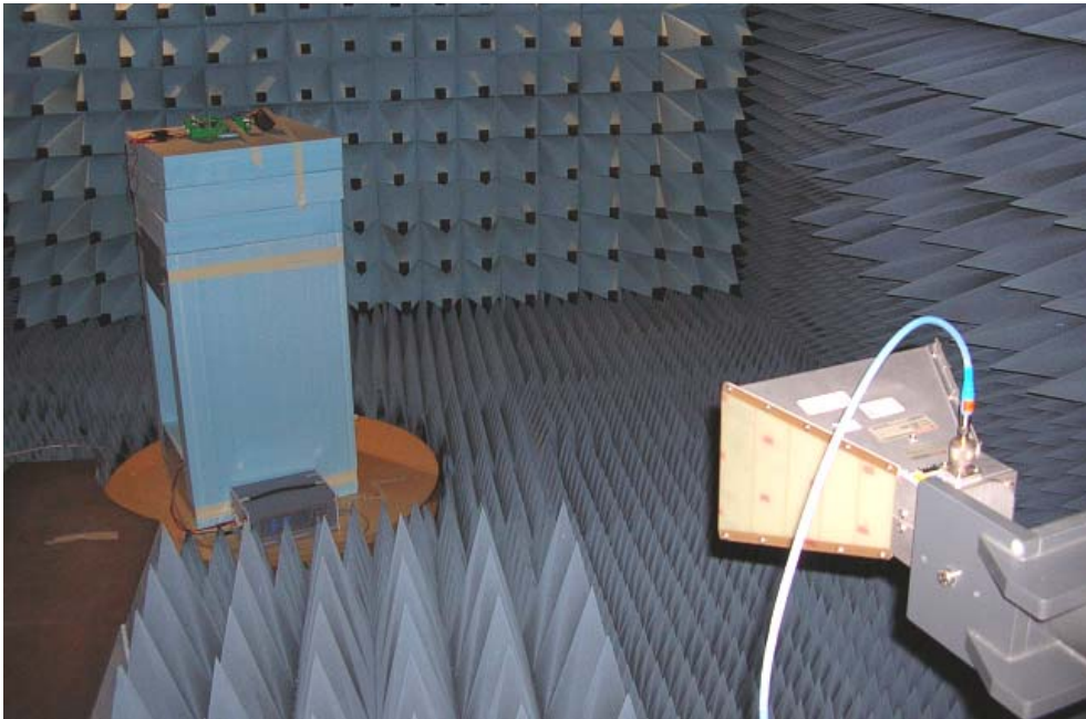
Radiated spurious emission 1-26 GHz
