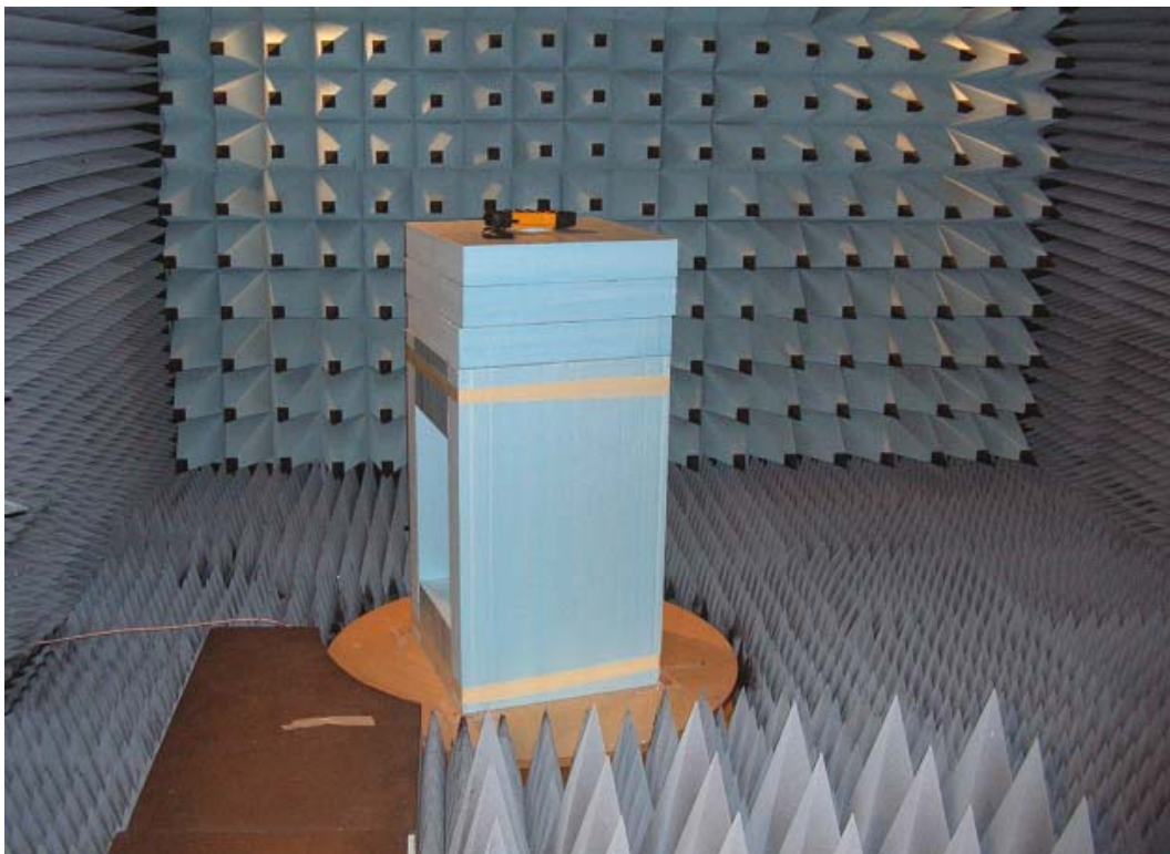
Radiated spurious emission 1-26 GHz
