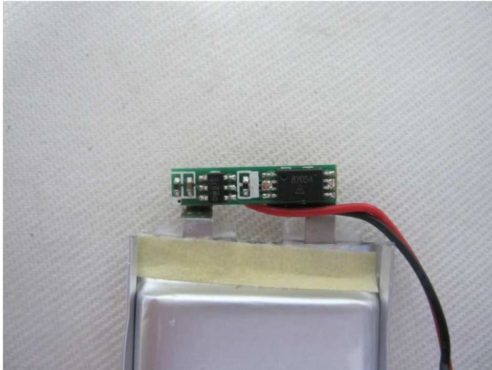
Fig. 7: Internal view
