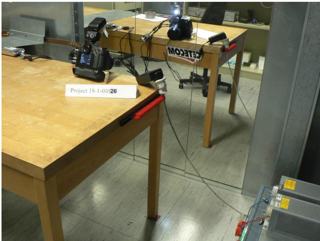
Photograph 1: Conducted measurements test set-up for AC-mains emission measurements
