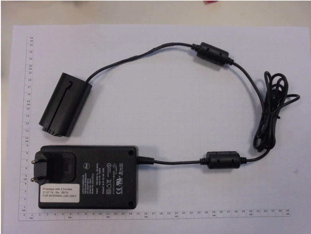
Photograph 5: Auxiliary equipment under test (AE 1), AC-Adapter S, Type ACA-SCL3
