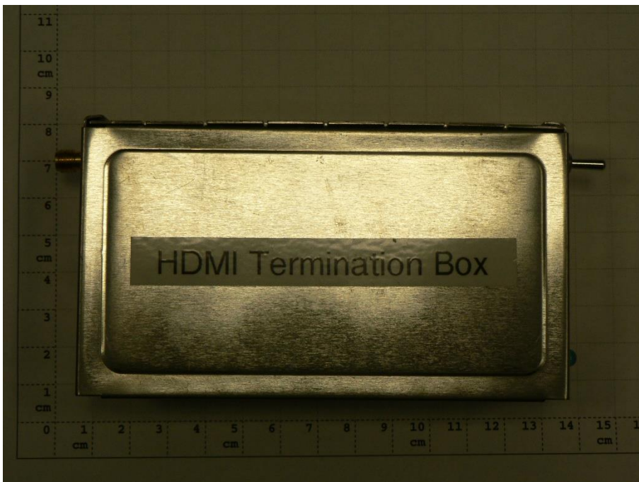
Photograph 12: Auxiliary equipment under test (AE 9), Termination Box 50Ohm, Type: for AE8
