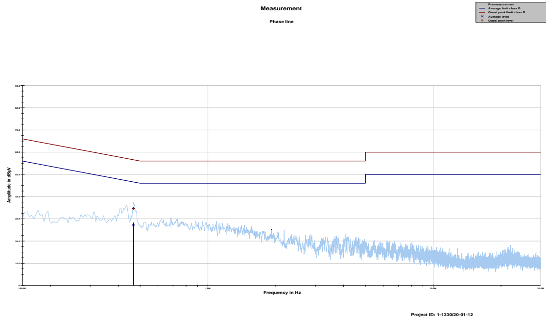
Plot 1: 150 kHz to 30 MHz, phase line
