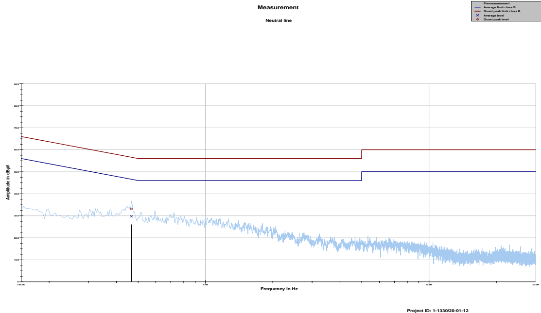
Plot 2: 150 kHz to 30 MHz, neutral line
