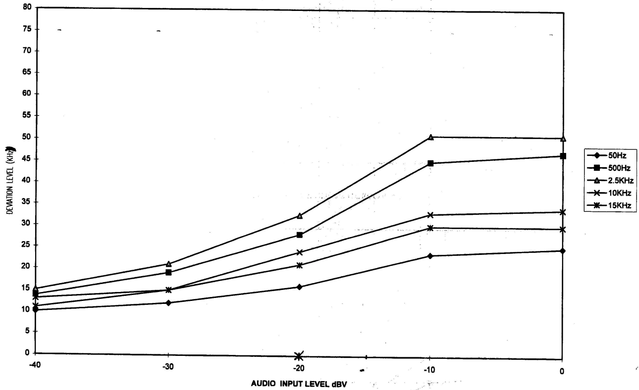
Sheet | Chart 1 (AUDIO INPUT LEVEL Vs DEVIATION)
