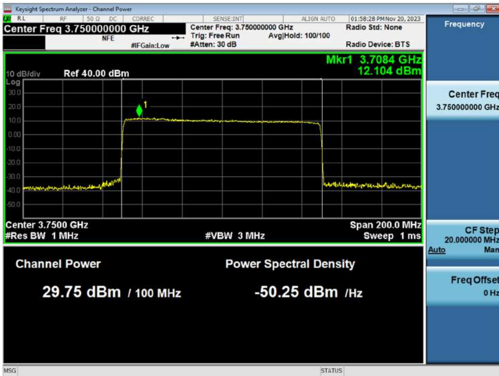
3 dB above the AGC threshold PSD / 3.7 GHz Service / Uplink / 5G NR 100 MHz
