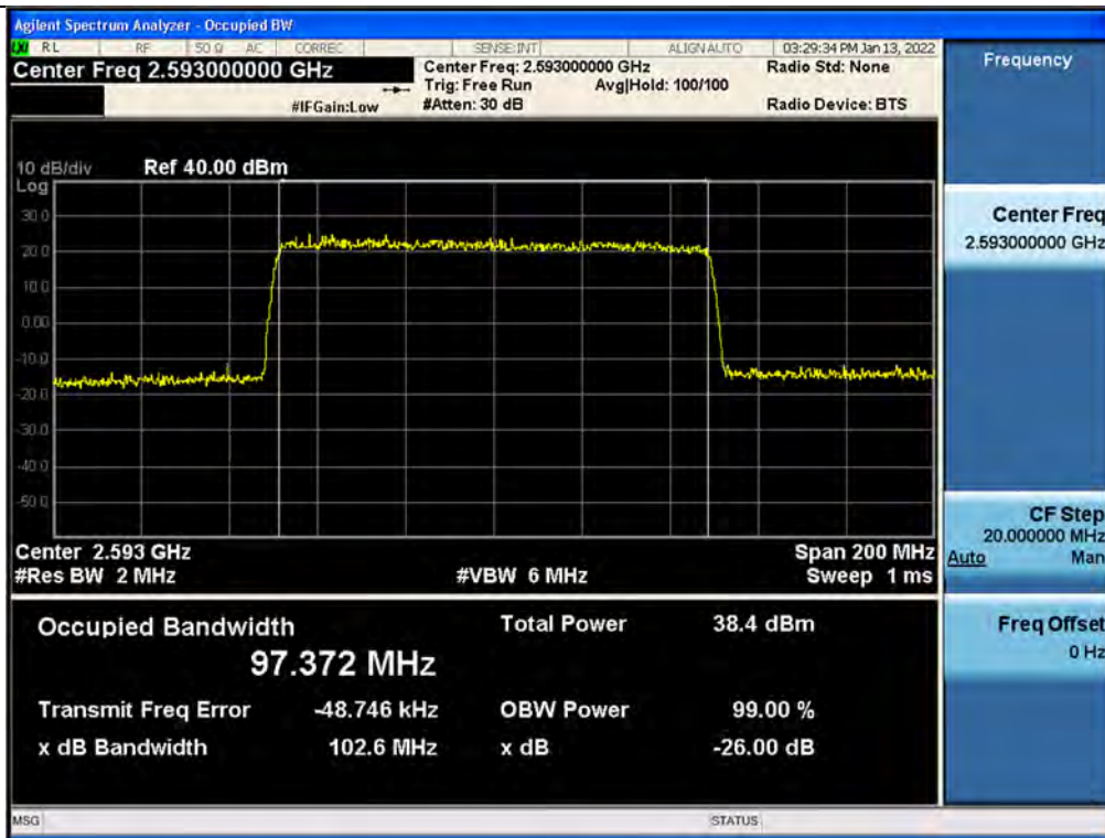
Output / BRS/EBS / Uplink / 5G NR 100 MHz
