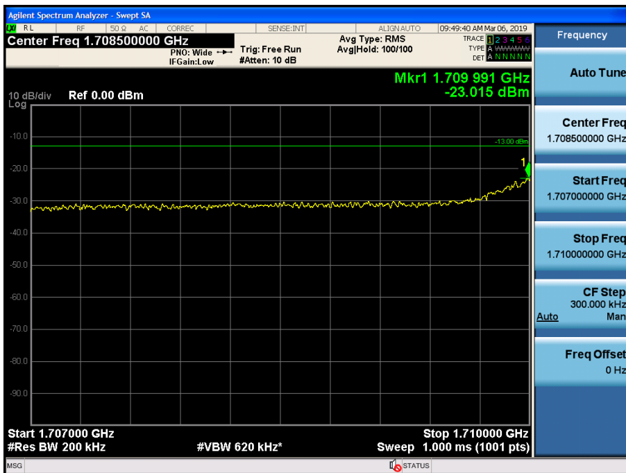
Out-of-band (two adjacent test signals) / AWS / Uplink / LTE 20 MHz / Lower
