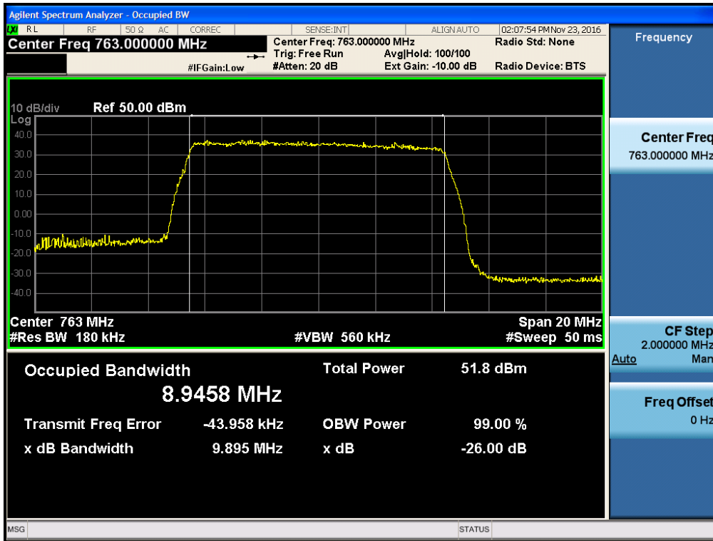
[700 Band AGC threshold Downlink Output LTE 10 MHz Middle]
