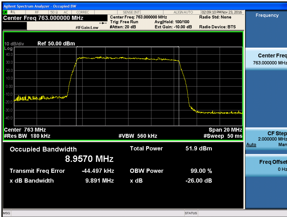
[700 Band +3 dB above the AGC threshold Downlink Output LTE 10 MHz Middle]
