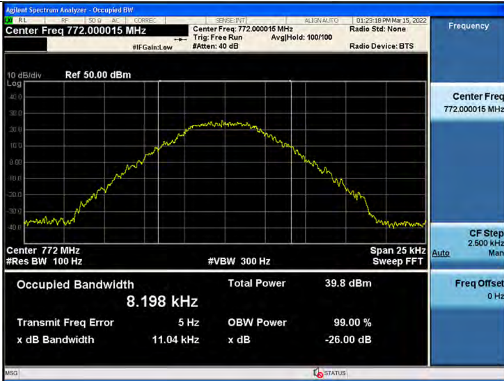
Output / PS Narrowband / Downlink / P25 Phase 1
