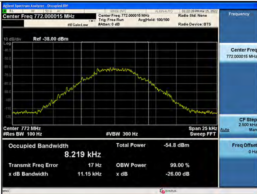
Input / PS Narrowband / Downlink / P25 Phase 1
