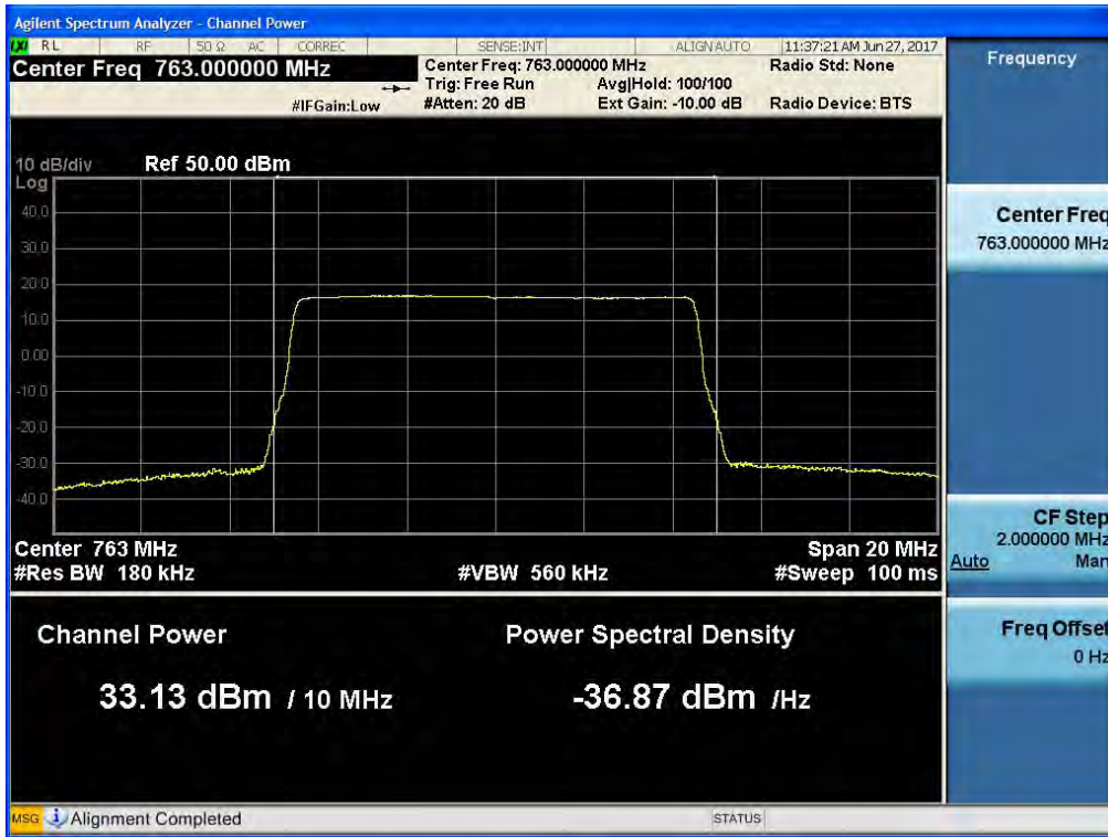
[AGC threshold Downlink - Middle]
