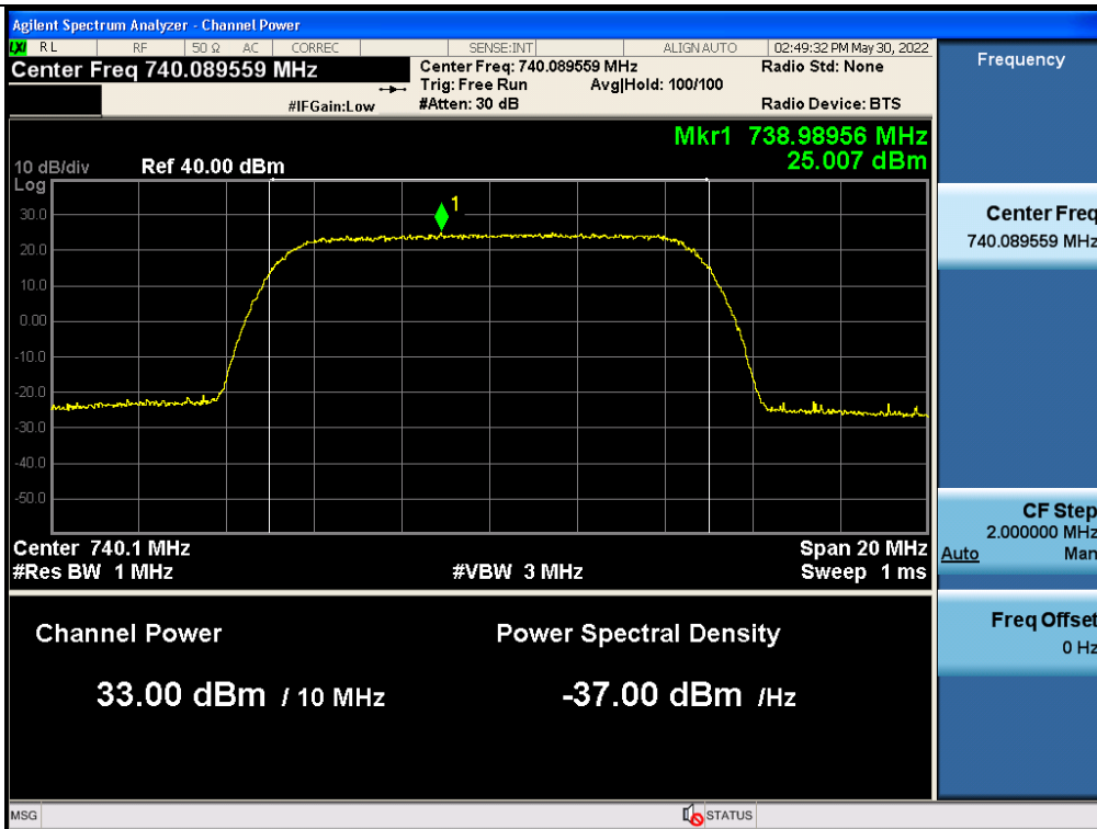
3 dB above the AGC threshold PSD / Lower 700 MHz / Downlink / LTE 10 MHz
