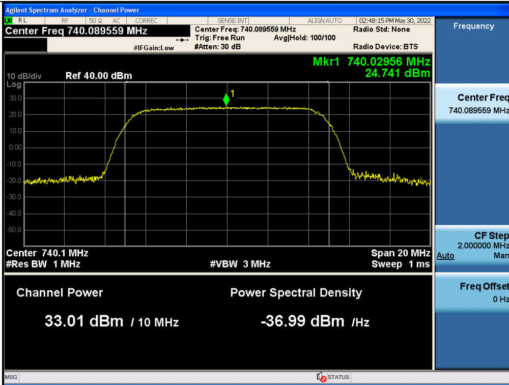
PSD / Lower 700 MHz / Downlink / LTE 10 MHz
