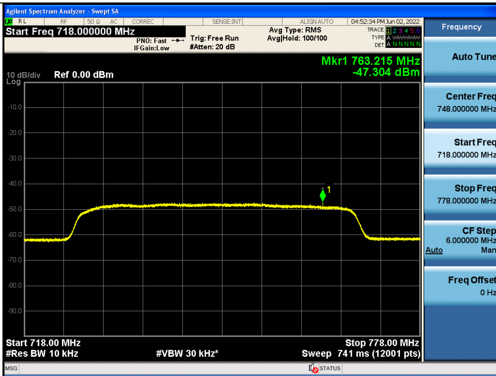
Noise Figure / FirstNet (758 ~ 768 MHz) / Downlink
