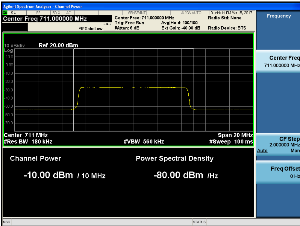
[AGC threshold Uplink - High]
