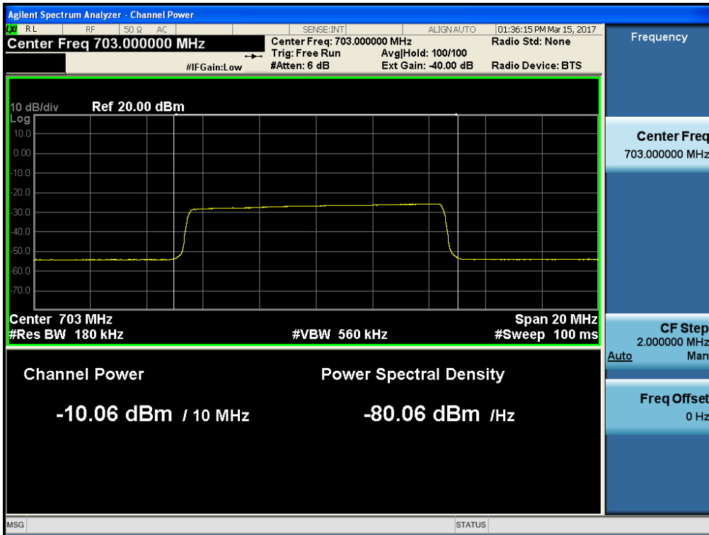
[AGC threshold Uplink - Low]
