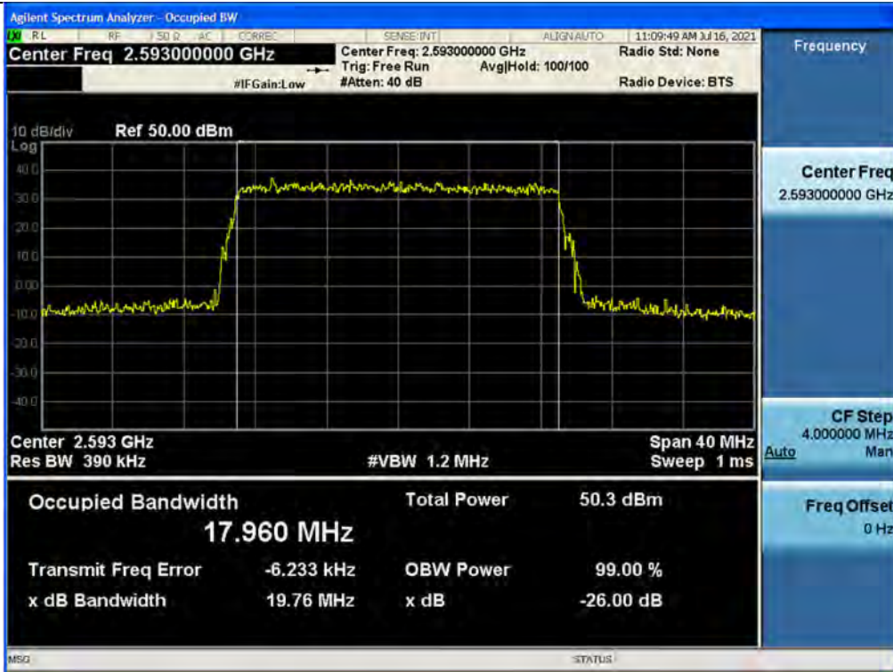
Output / BRS/EBS / Downlink / LTE 20MHz
