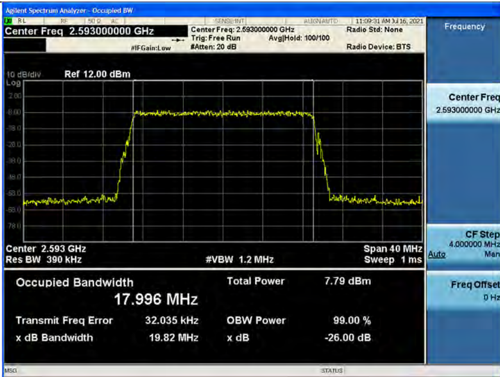
Input / BRS/EBS / Downlink / LTE 20 MHz
