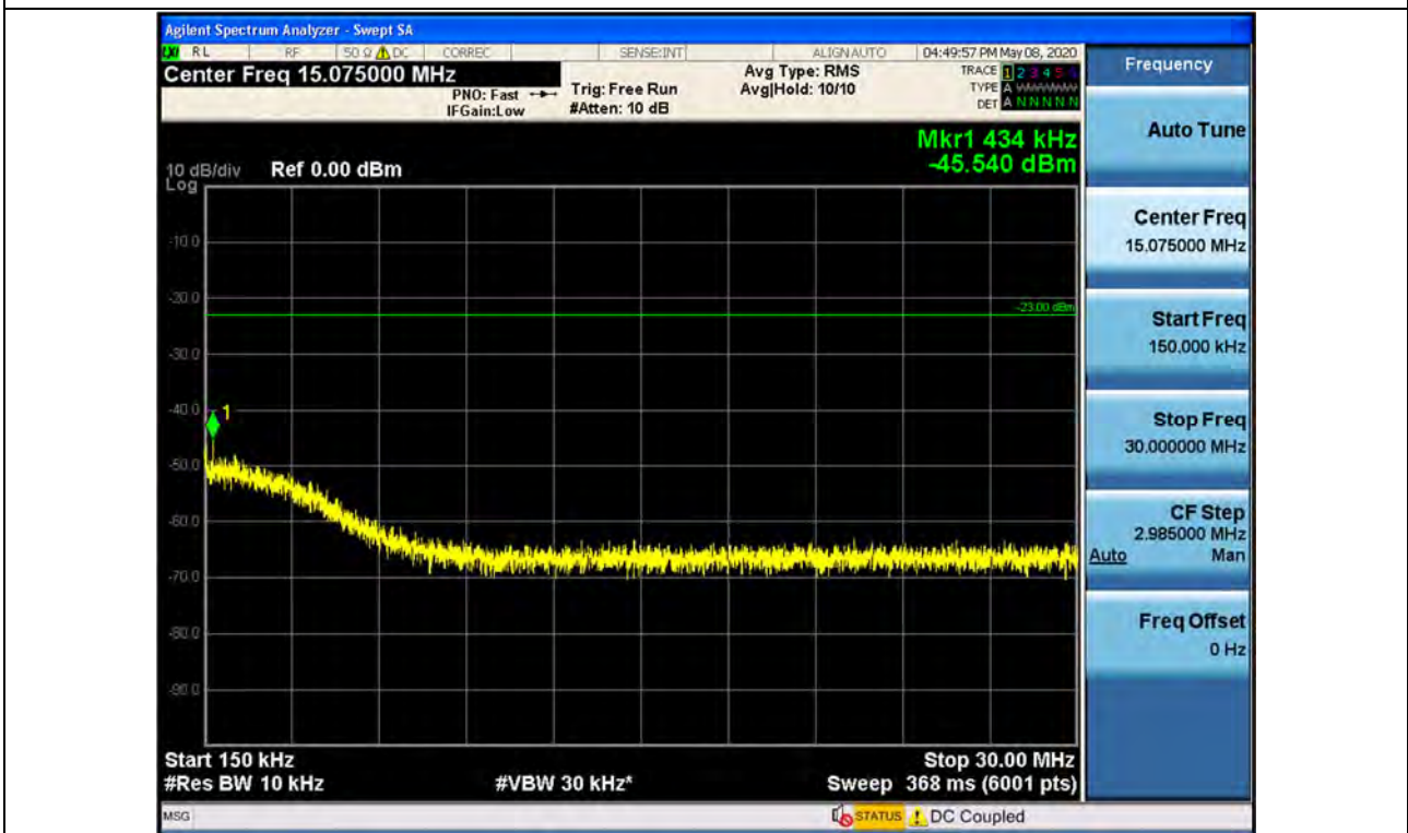
Spurious / Lower 700 MHz / Downlink/ LTE 10 MHz / Low / 150 kHz ~ 30 MHz
