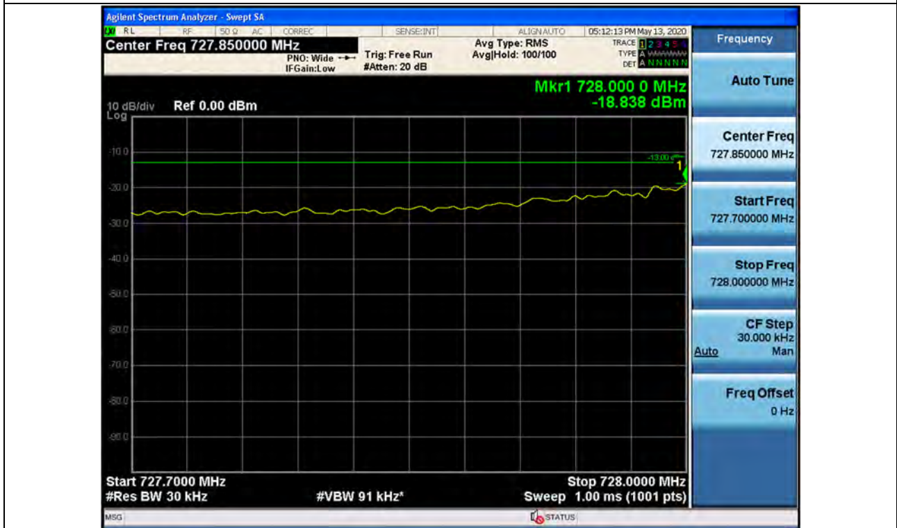
Out-of-band (single test signals) / Lower 700 MHz / Downlink / LTE 10 MHz / Lower
