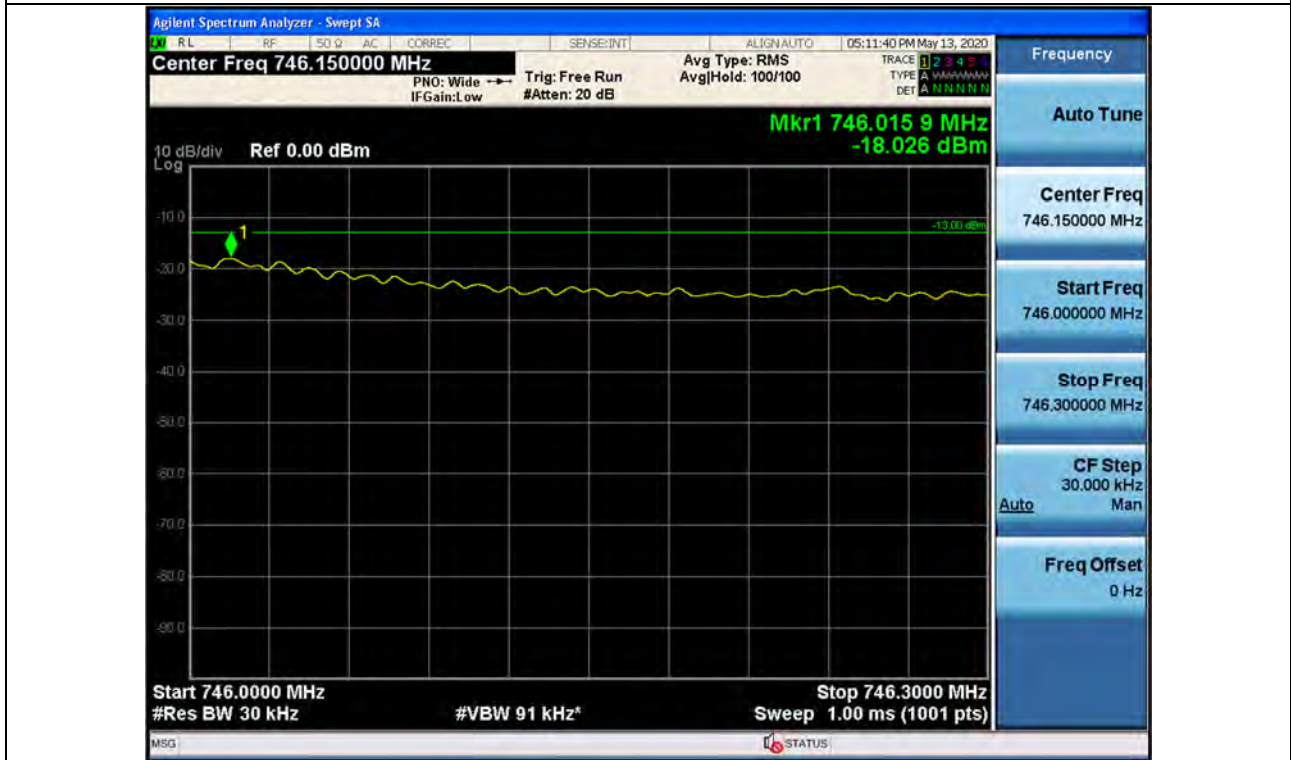
Out-of-band (single test signals) / Lower 700 MHz / Downlink / LTE 10 MHz / Upper
