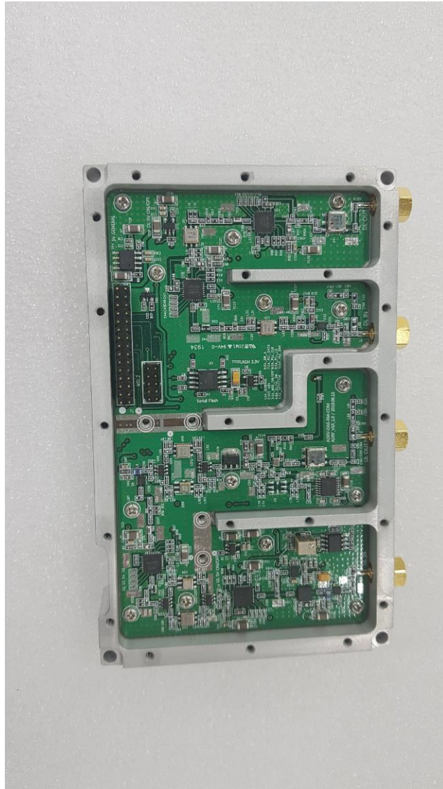
[COM Module-7FN]
