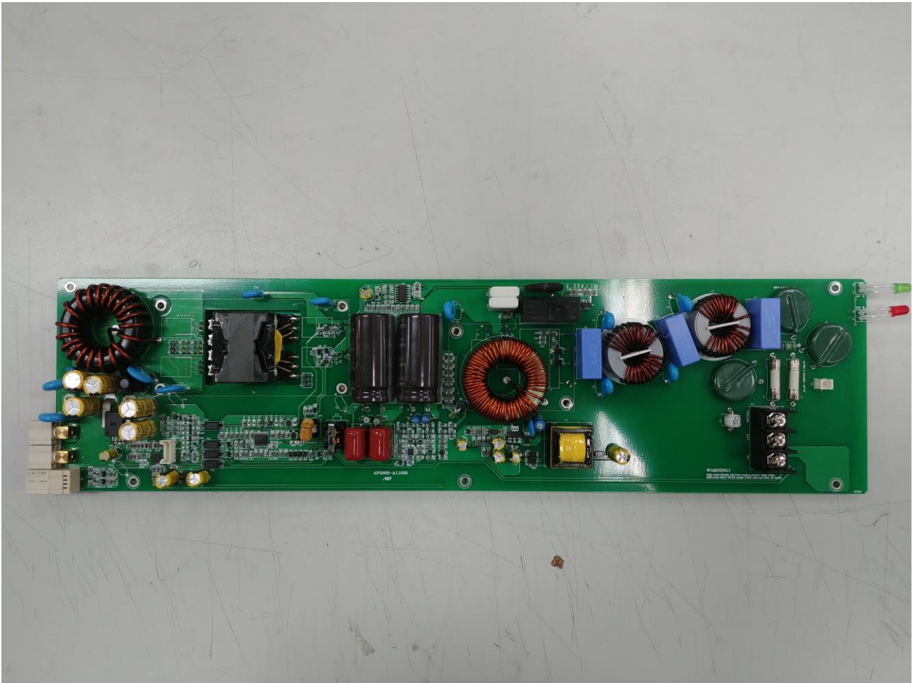
[RU PSU-AC Internal photo-1]
