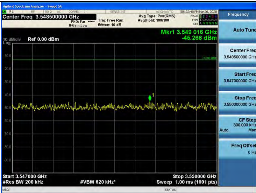
+3 dB above Out-of-band (single test signals) / CBRS / Downlink / LTE 20 MHz / Lower
