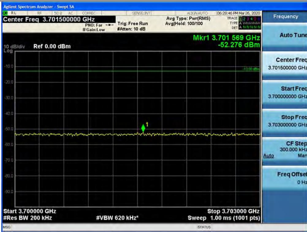
+3 dB above Out-of-band (single test signals) / CBRS / Downlink / LTE 20 MHz / Upper
