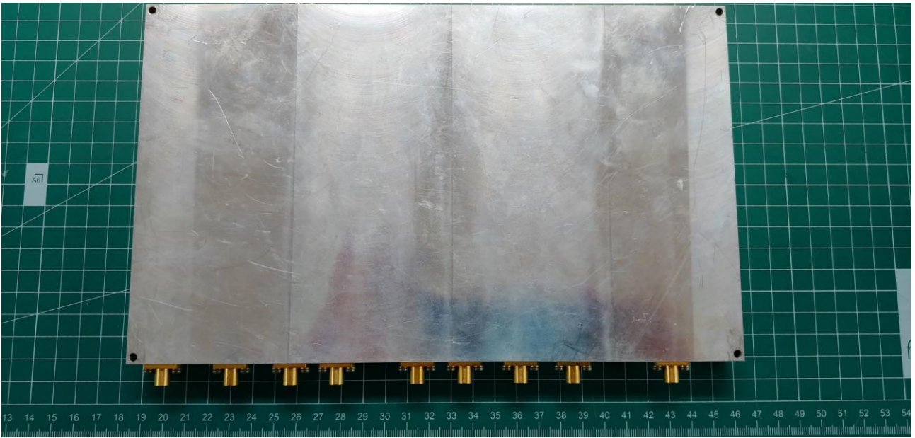
[ADX-DLPR Multiplexer (bottom)]
