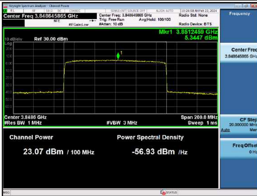
3 dB above the AGC threshold PSD / 3.7 GHz Service / Downlink / Ant. 1 / 5G NR 100 MHz
