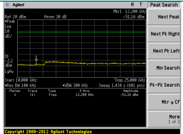
10GHz~25GHz
