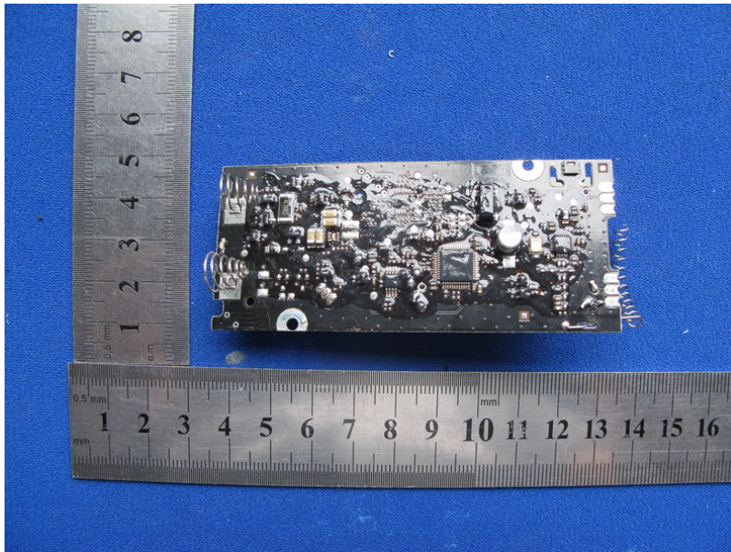
Photo 18 Appearance of PCB (Indoor)
