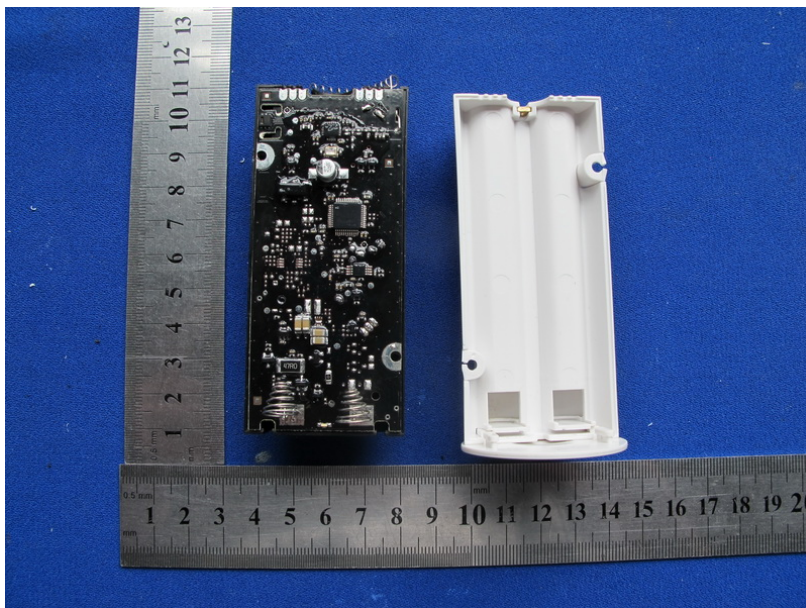
Photo 17 Internal of EUT (Indoor)
