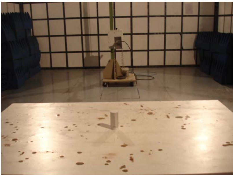
Photo of Setup for Radiated Emission (Indoor) (Above 1 GHz)
