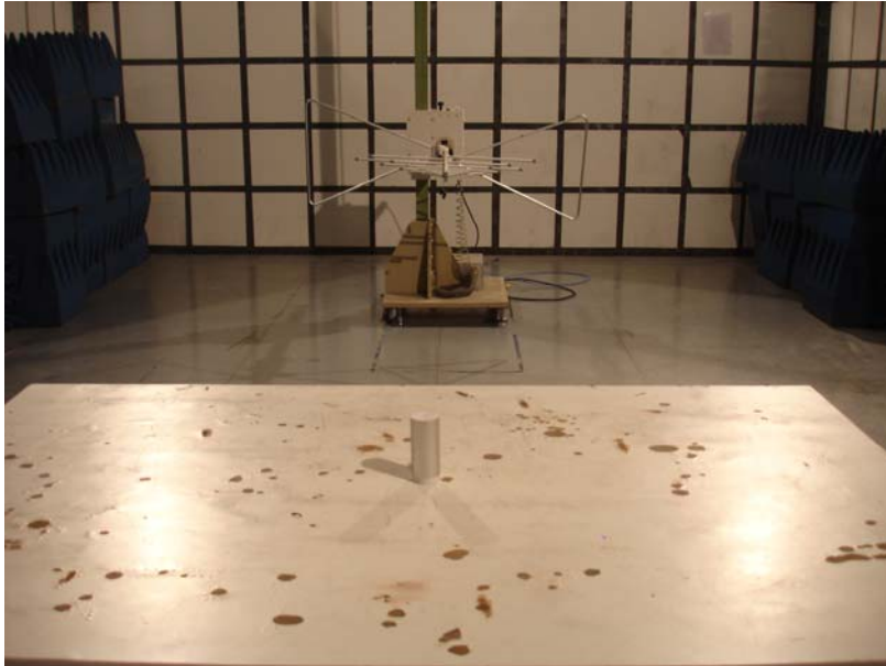
Photo of Setup for Radiated Emission (Indoor) (Bellow 1 GHz)
