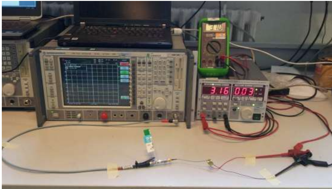
Test setup for radio conducted tests
