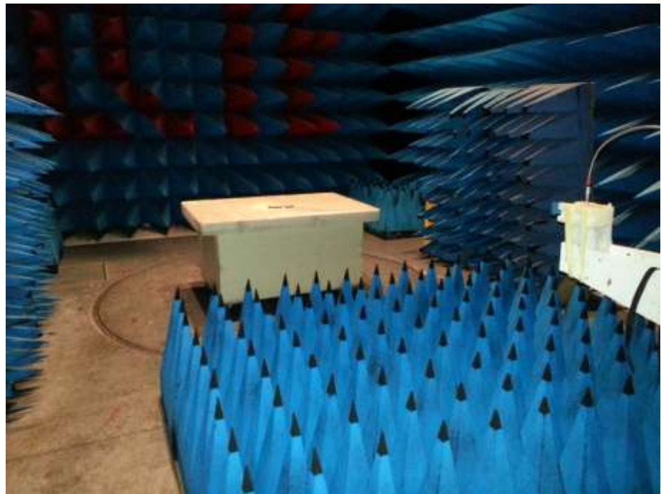
Test setup for radiated field strength
