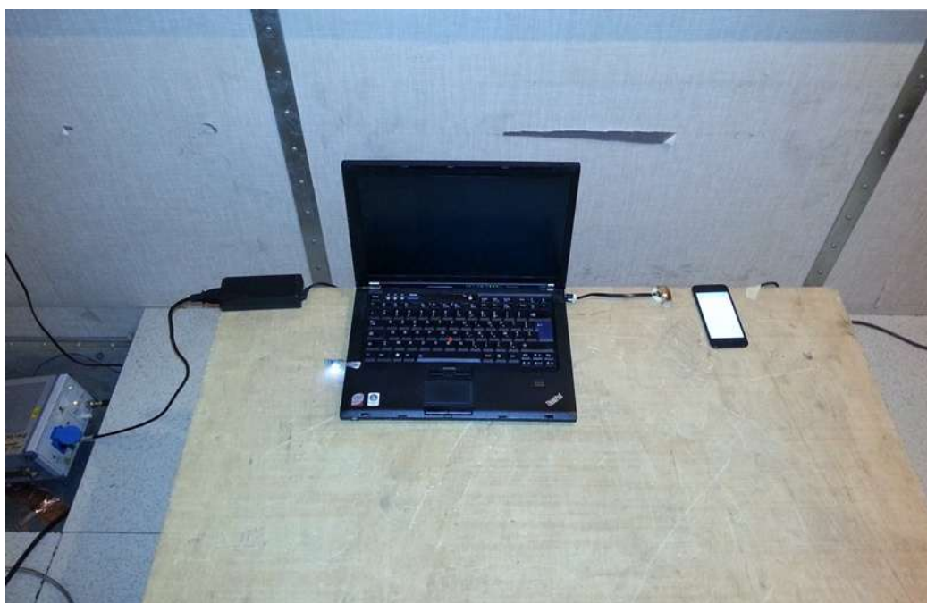
Test setup for power line conducted emissions
