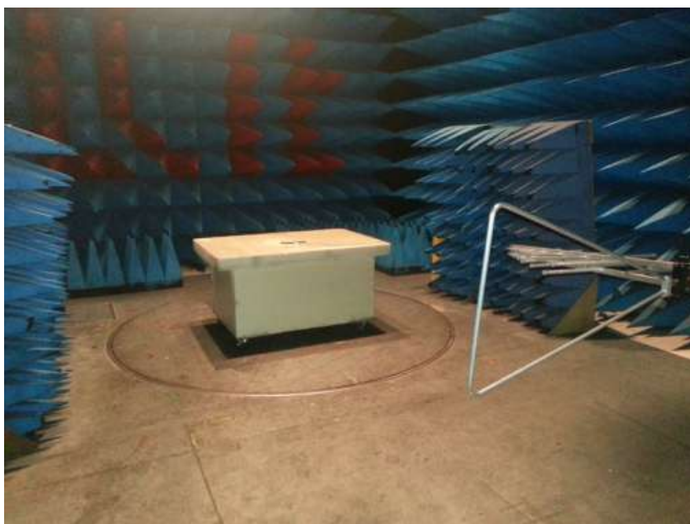
Test setup for radiated field strength
