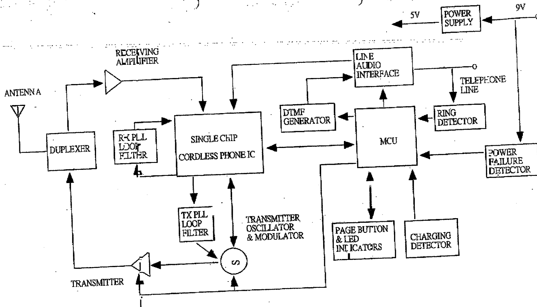
BASE UNIT BLOCK DIAGRAM
