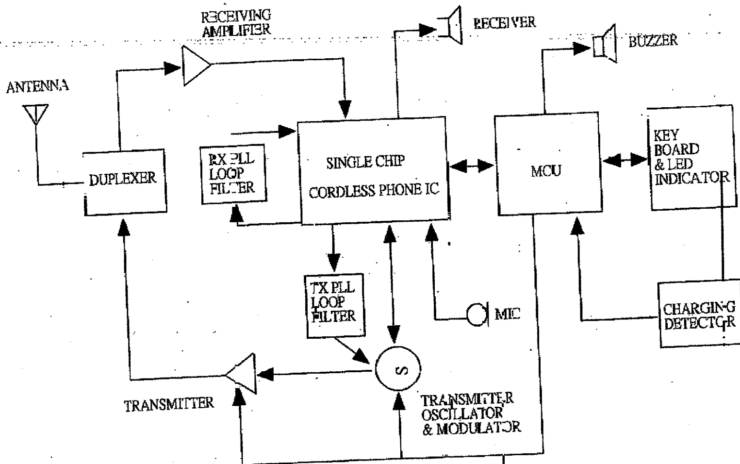
HEADSET BLOCK DIAGRAM
