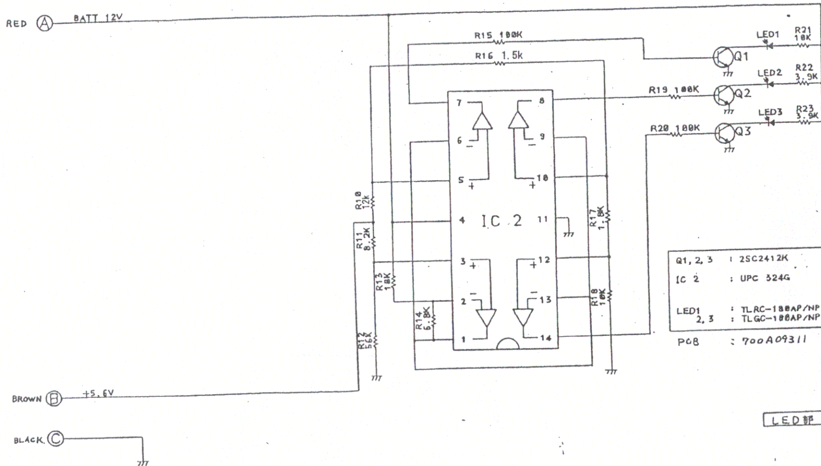
CIRCUIT DIAGRAM
