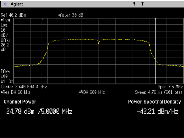
2440MHz_5MHz BW_Output Power_Port 1
