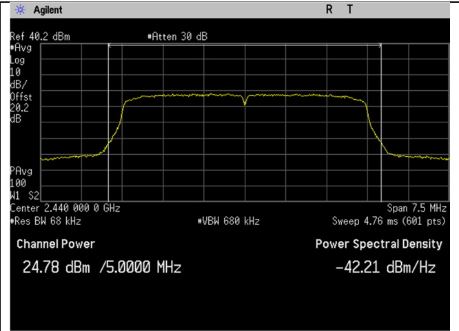
2440MHz_5MHz BW_Output Power_Port 2
