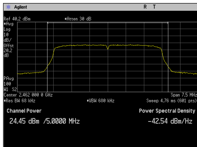
2462MHz_5MHz BW_Output Power_Port 1
