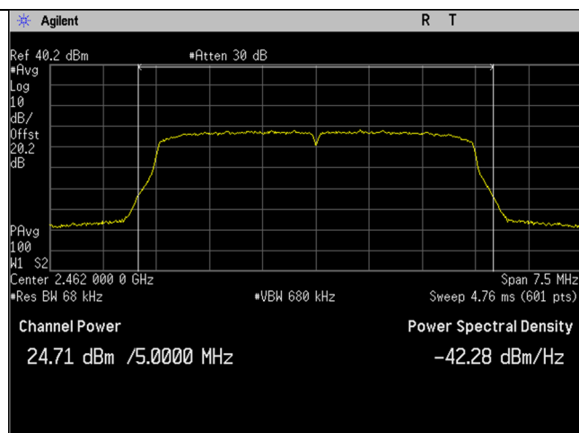
2462MHz_5MHz BW_Output Power_Port 2
