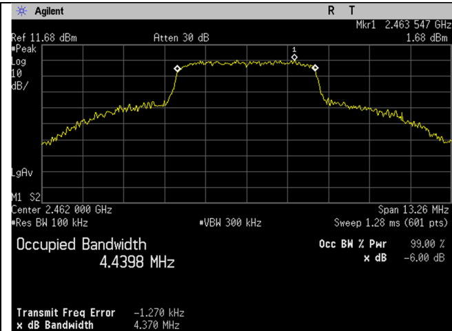
2462MHz_5MHz BW_Occupied Bandwidth_- 6dB_Port 1
