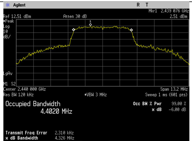
2440MHz_5MHz BW_Occupied Bandwidth_99 percent_Port 2
