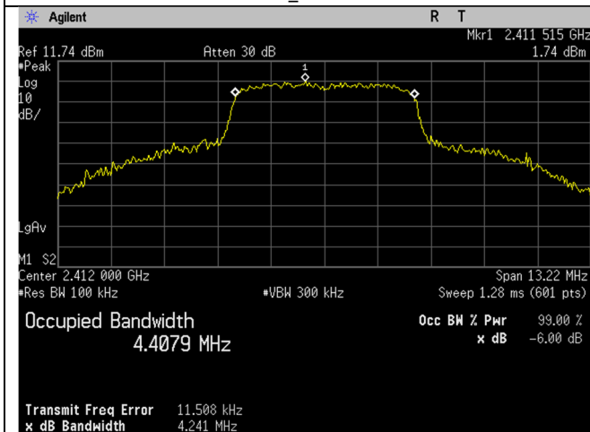
2412MHz_5MHz BW_Occupied Bandwidth_6dB_Port 2
