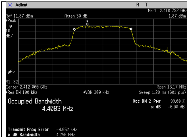
2412MHz_5MHz BW_Occupied Bandwidth_6dB_Port 1
