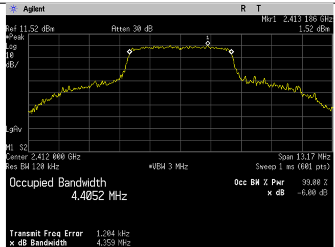
2412MHz_5MHz BW_Occupied Bandwidth_99 percent_Port 1
