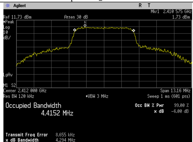
2412MHz_5MHz BW_Occupied Bandwidth_99 percent_Port 2
