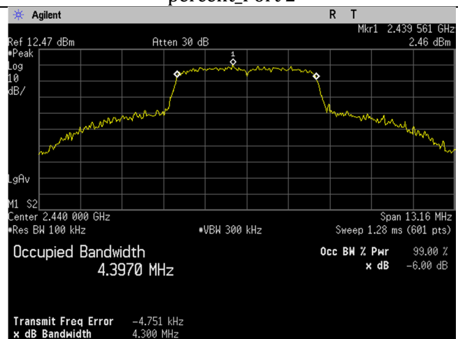
2440MHz_5MHz BW_Occupied Bandwidth_6dB_Port 2
