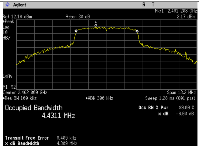
2462MHz_5MHz BW_Occupied Bandwidth_- 6dB_Port 2
