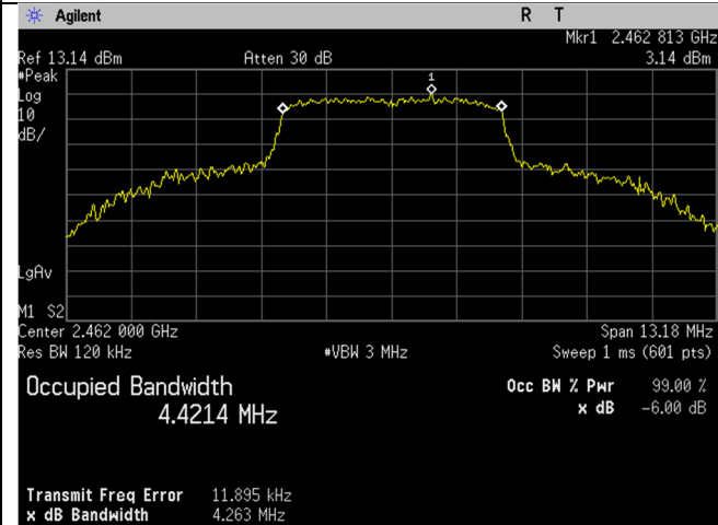
2462MHz_5MHz BW_Occupied Bandwidth_99 percent_Port 1
