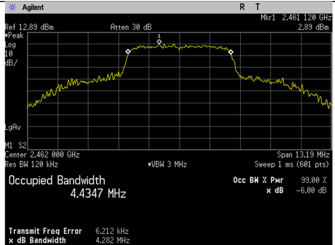
2462MHz_5MHz BW_Occupied Bandwidth_99 percent_Port 2
