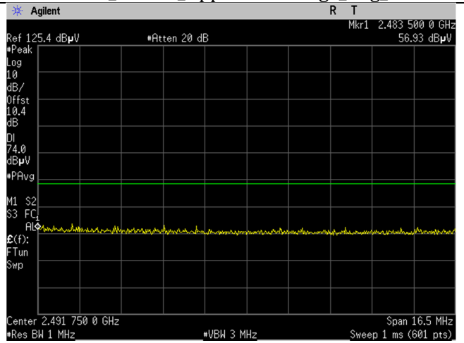
2462MHz_15.209_Upper Band Edge_Avg_Port 1
