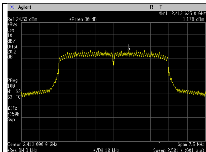
2412MHz_5MHz BW_Spectral Density_Port 1
