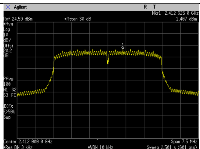
2412MHz_5MHz BW_Spectral Density_Port 2
