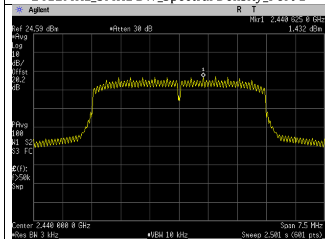
2440MHz_5MHz BW_Spectral Density_Port 1
