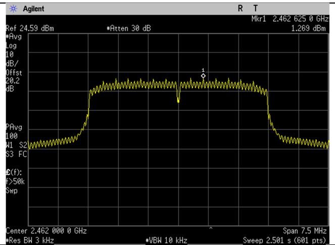
2462MHz_5MHz BW_Spectral Density_Port 2
