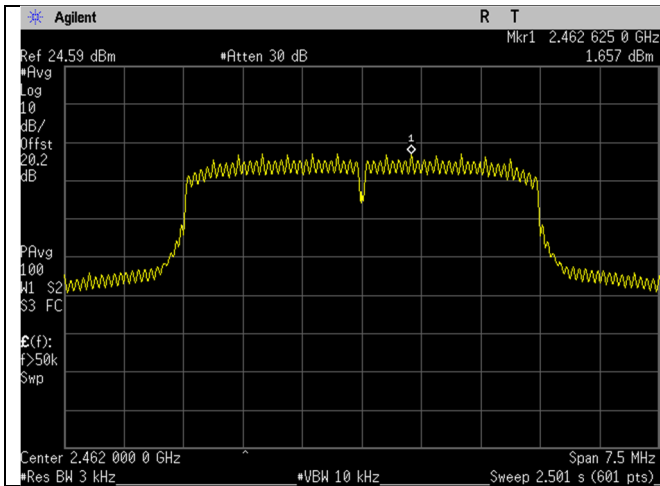
2462MHz_5MHz BW_Spectral Density_Port 1
