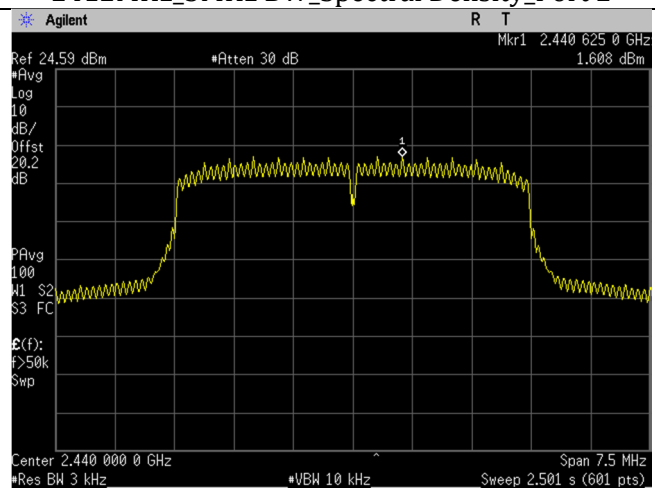
2440MHz_5MHz BW_Spectral Density_Port 2
