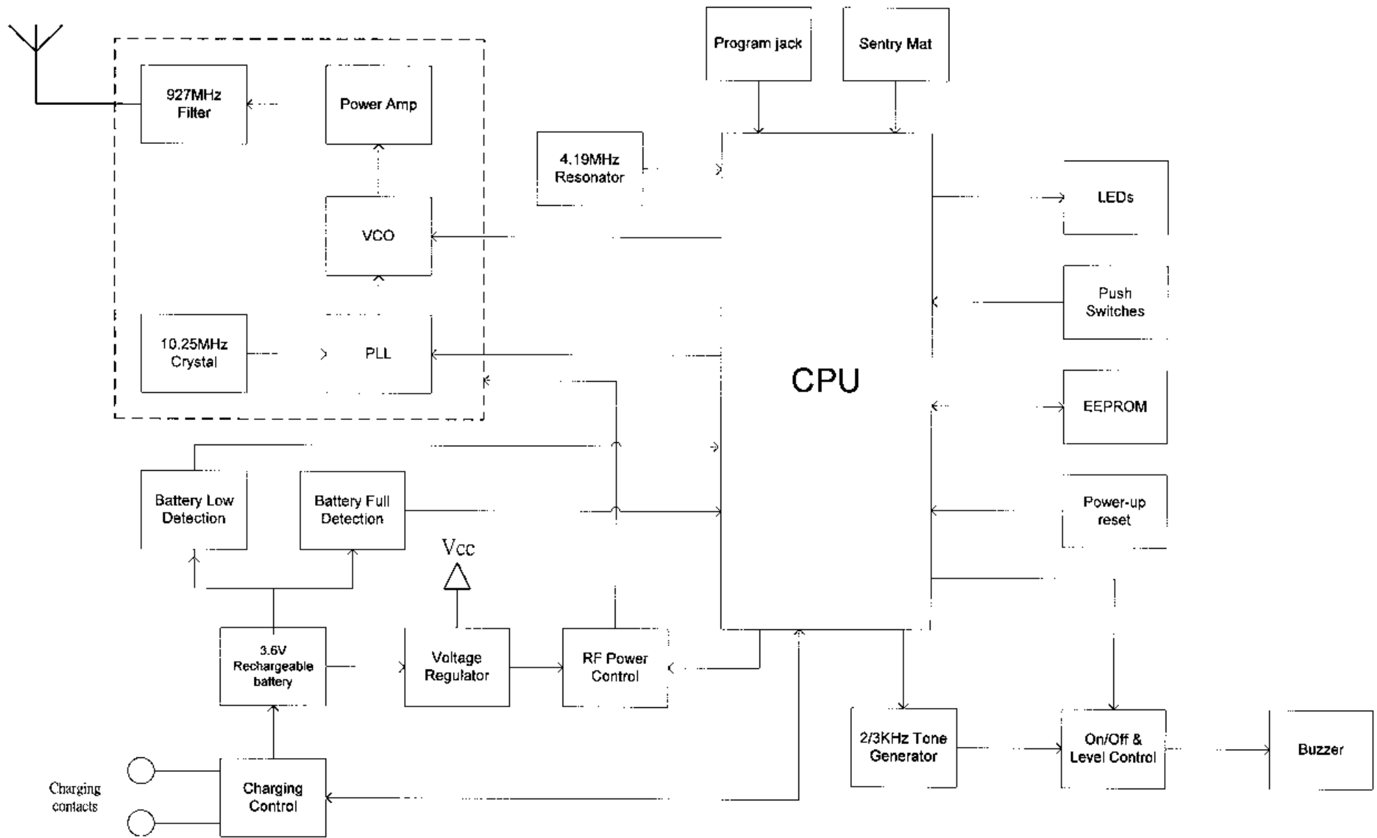
Block diagram of Transmit unit
