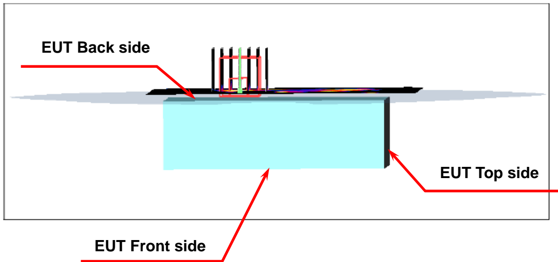
Figure 5. Body SAR Test Setup (Flat Section)
