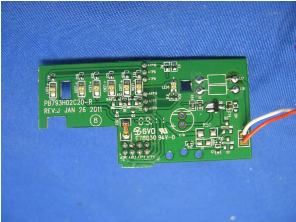
Parent Unit Another Main PCB comp side
