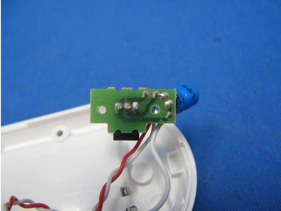
Parent Unit AC Jack Rear side
