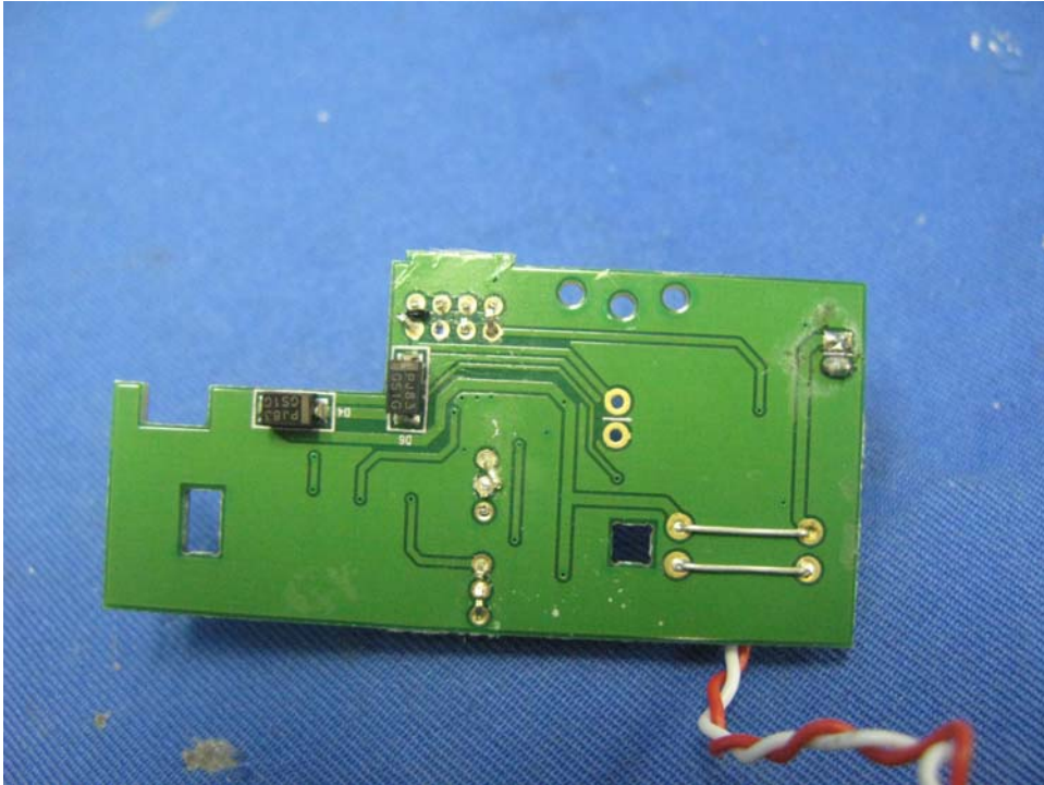
Parent Unit Another Main PCB solder side
