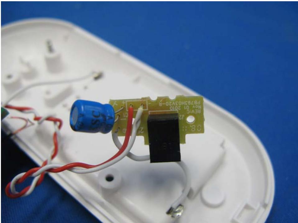
Parent Unit AC Jack Front side
