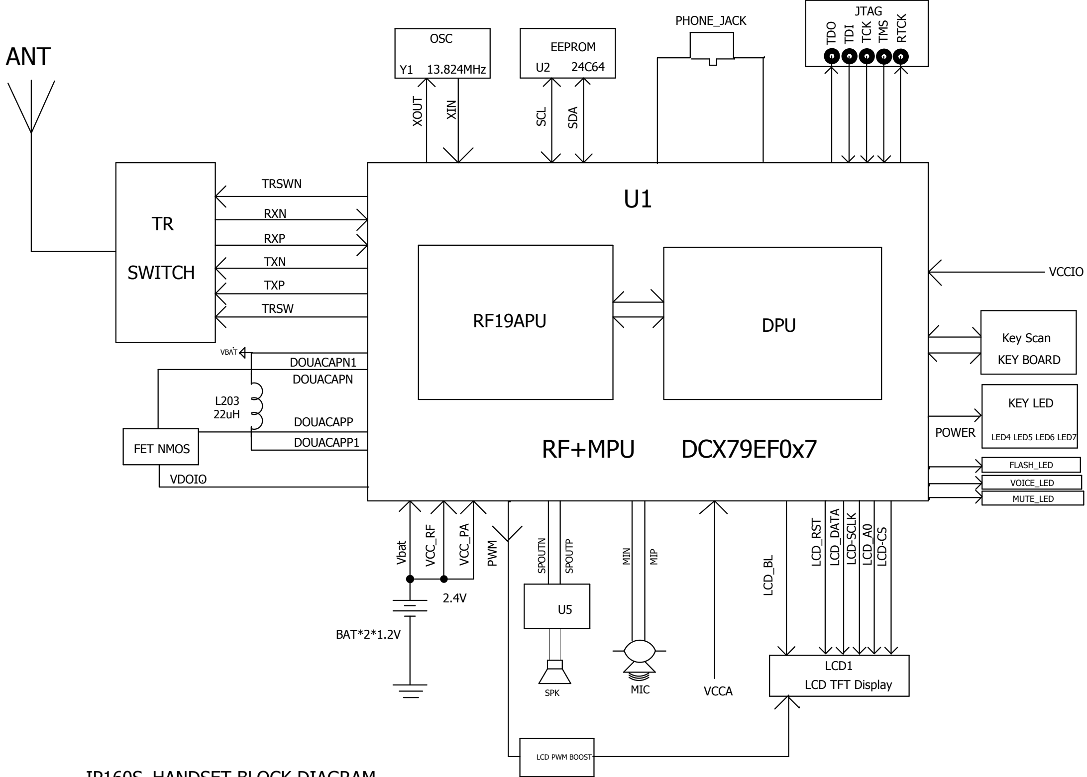
IP160S_HANDSET BLOCK DIAGRAM
