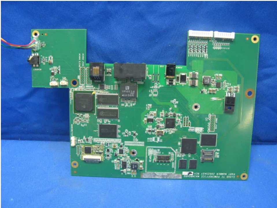
IP Phone Main PCB comp side
