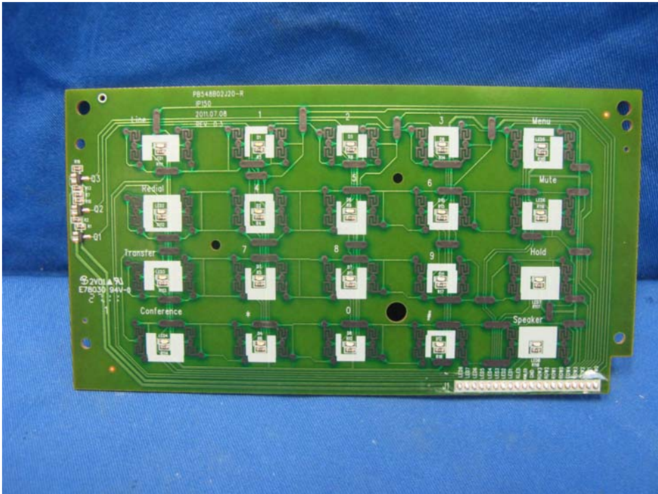
IP Phone Keypad front side
