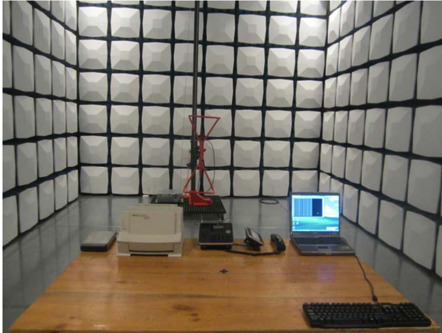
Radiated Emission - Rear View (IP125-TC-POE Mode)
