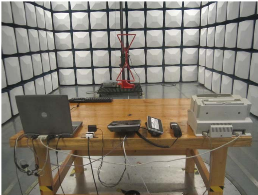
Radiated Emission - Rear View (IP125-TC-Adapter Mode)
