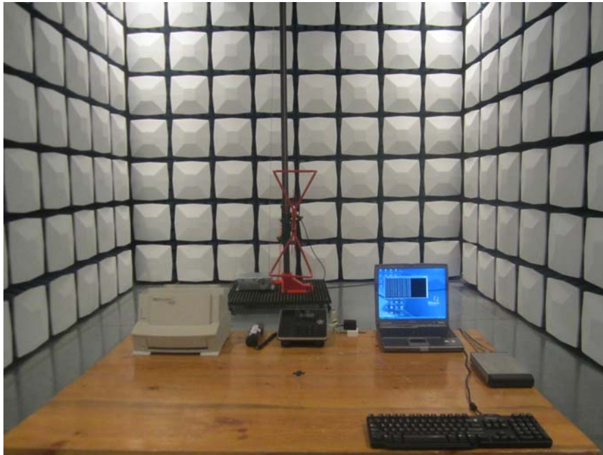
Radiated Emission - Rear View (IP115-TC-Adapter Mode)
