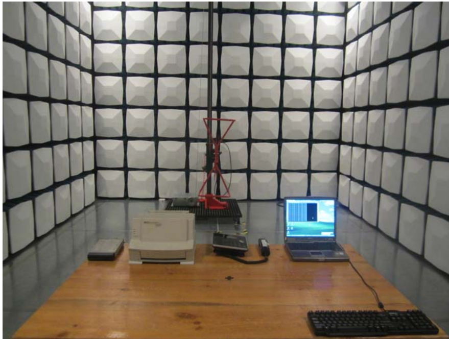
Radiated Emission - Rear View (IP115-TC-POE Mode)
