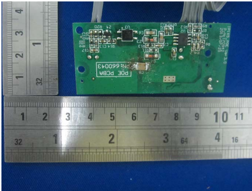
EUT -Host 660043 Top View
