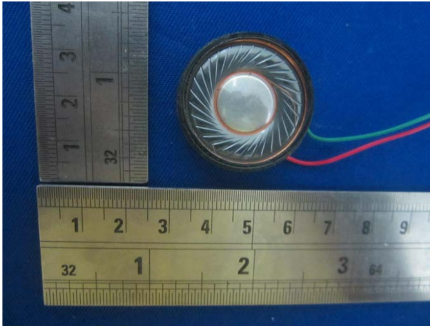
EUT –Microphone Speaker Bottom View
