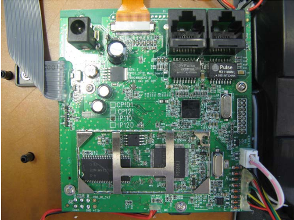
Desk Phone Main PCB comp side (View 1)
