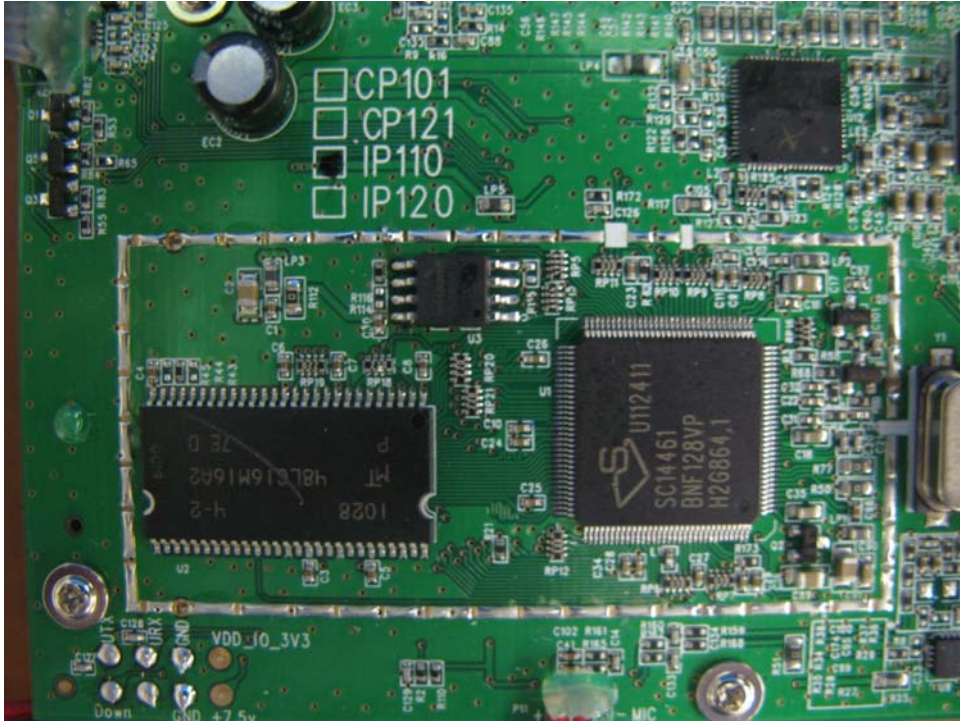
Desk Phone Oscillator PCB comp side
