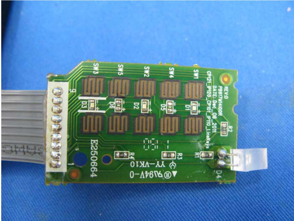
Desk Phone Page Key front side
