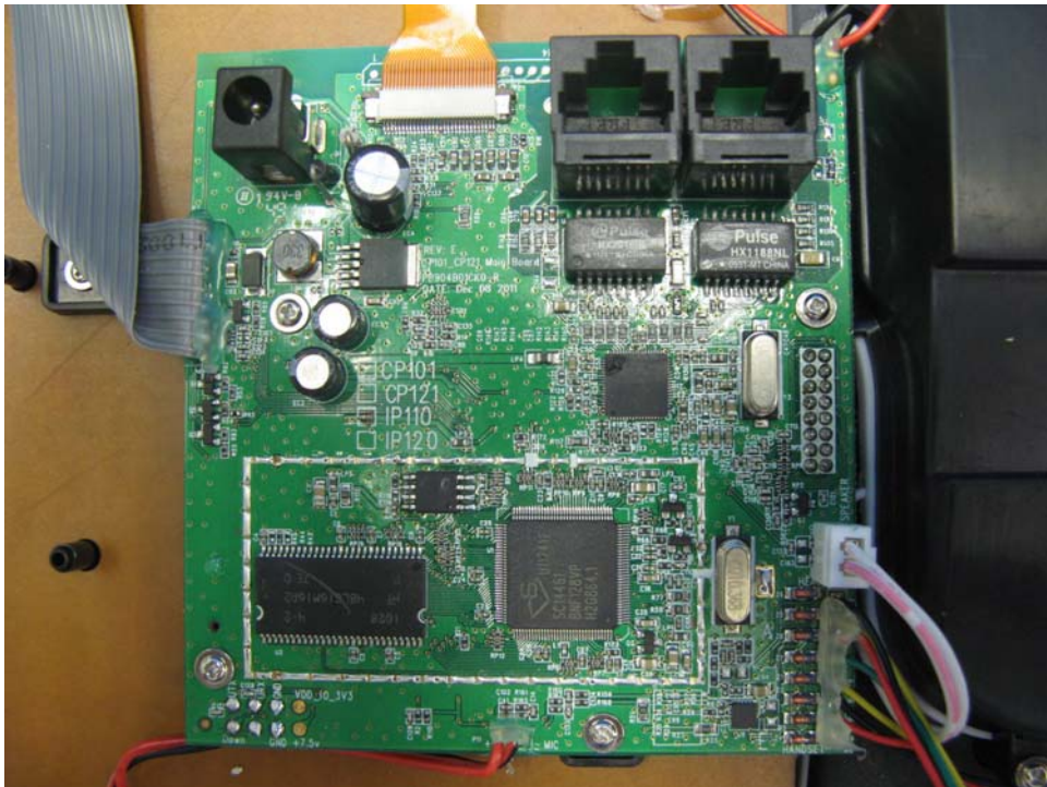
Desk Phone Main PCB comp side (View 2)
