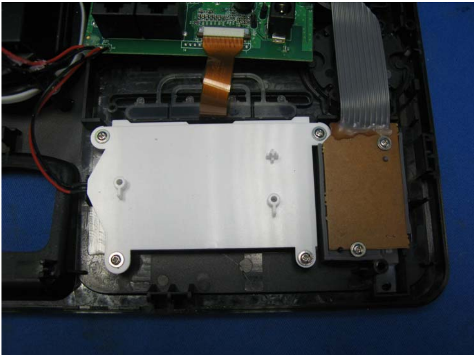
Desk Phone LCD Display rear side
