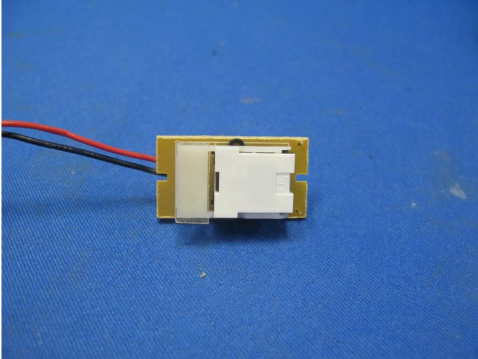
Desk Phone On/Off Hook front side
