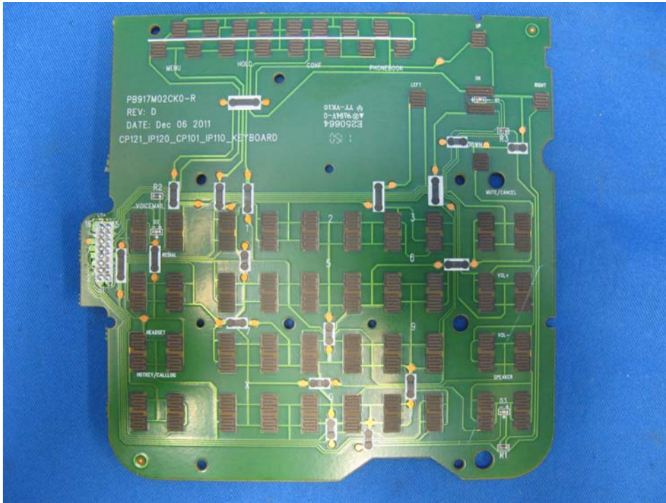
Desk Phone Keypad front side
