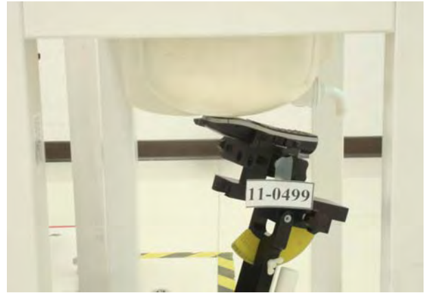
Figure 3. Right Head SAR Test Setup (Tilted)
