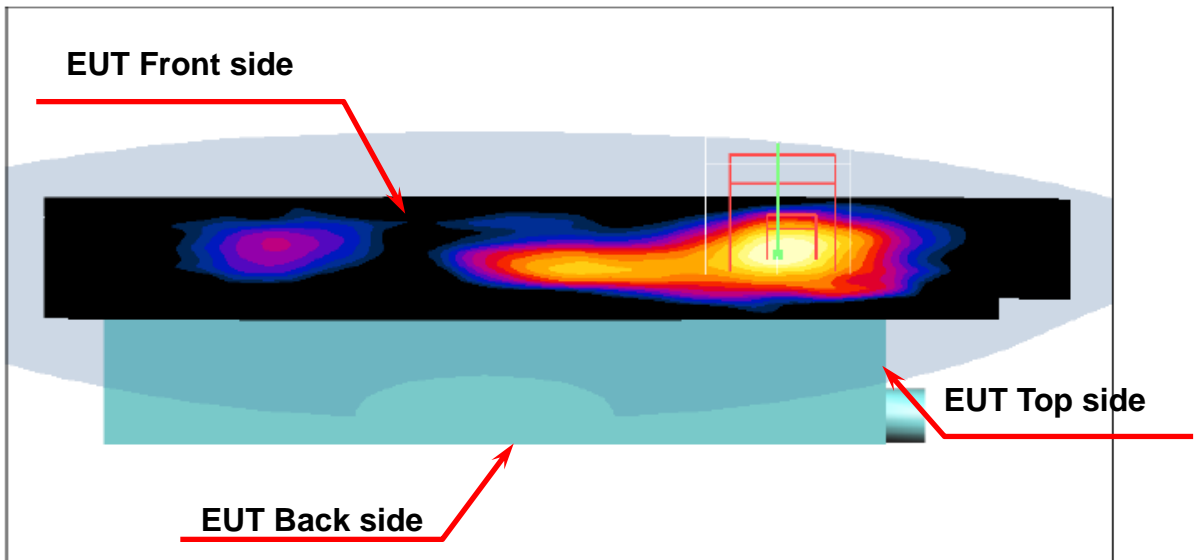
Figure 6. Body SAR Test Setup (Flat Section)
