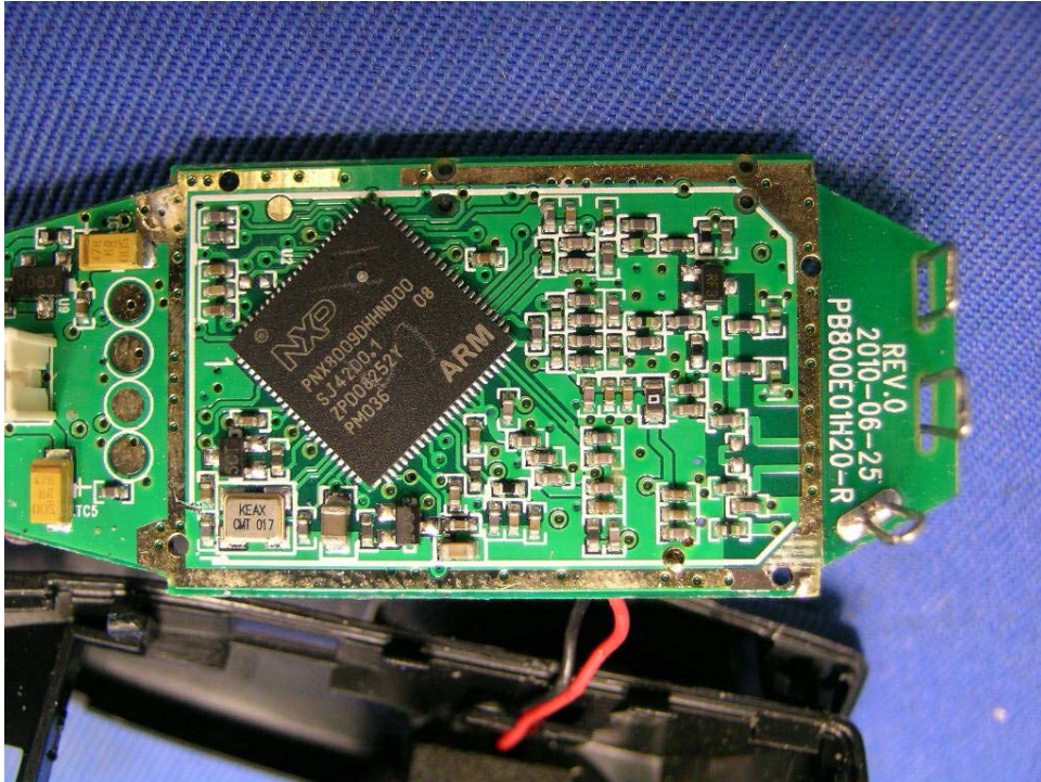
Headset Unit Oscillator PCB comp side
