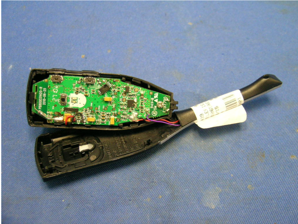
Headset Unit assembly (View 1)
