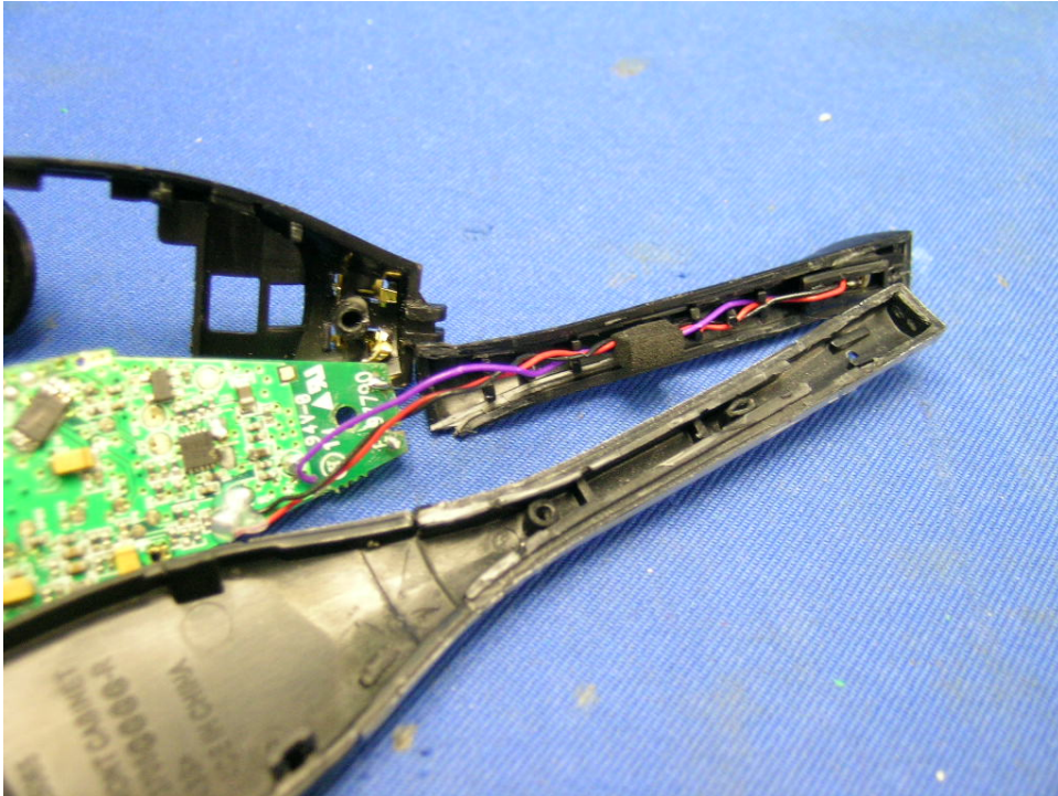
Headset Unit assembly (View 3)
