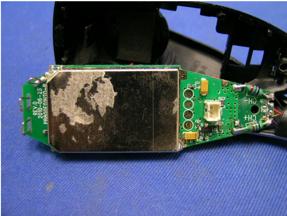
Headset Unit Main PCB comp side
