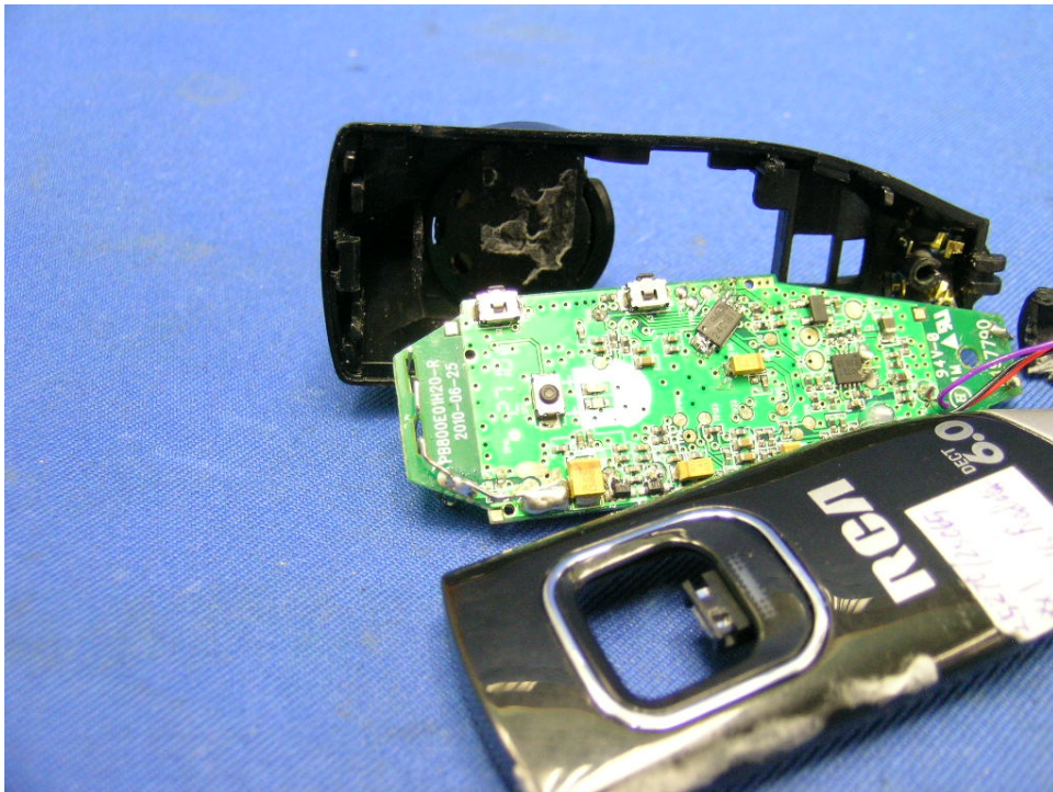
Headset Unit assembly (View 2)
