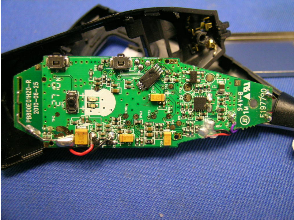
Headset Unit Main PCB solder side
