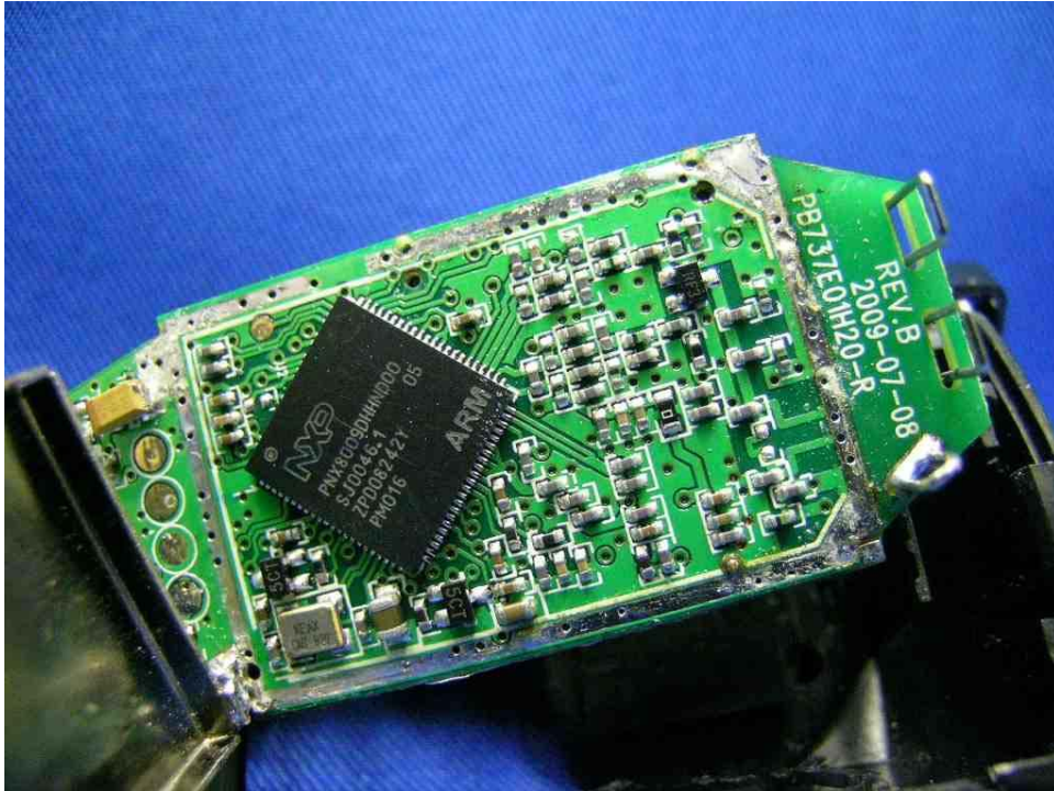
Cordless Headset RF module
