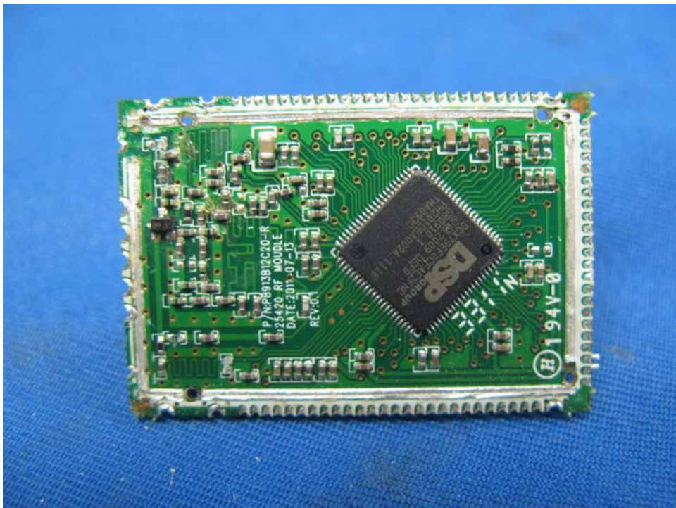
Base Unit RF Module comp side
