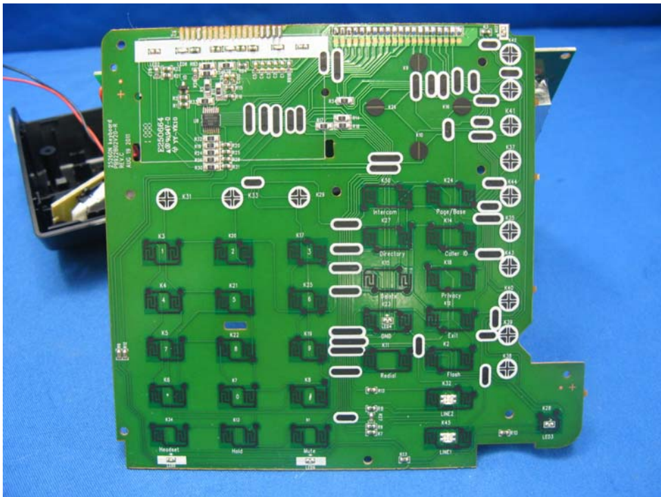
Base Unit Keypad and Display front side (View 2)
