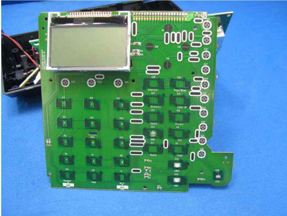
Base Unit Keypad and Display front side (View 1)
