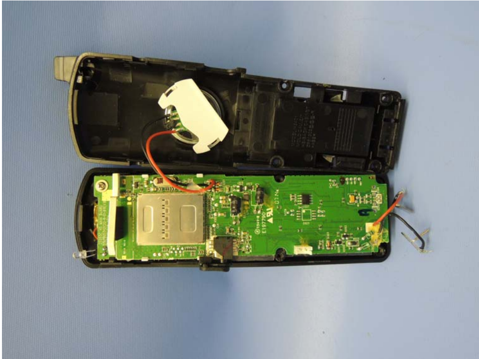
Handset assembly
