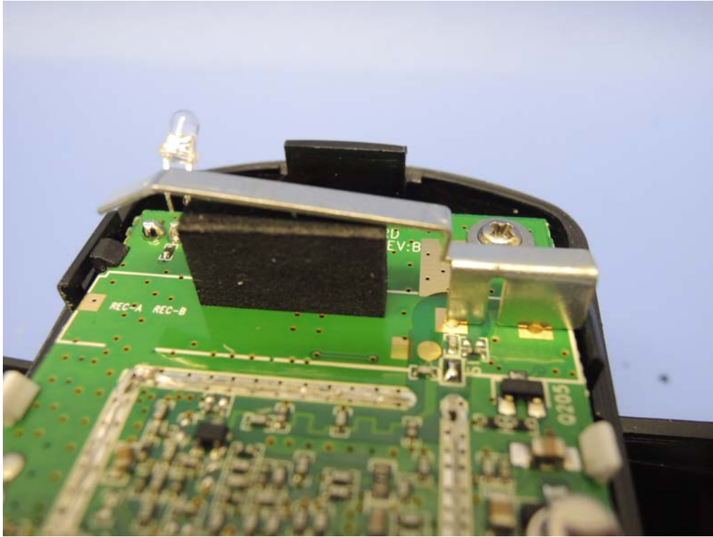
Handset Antenna
