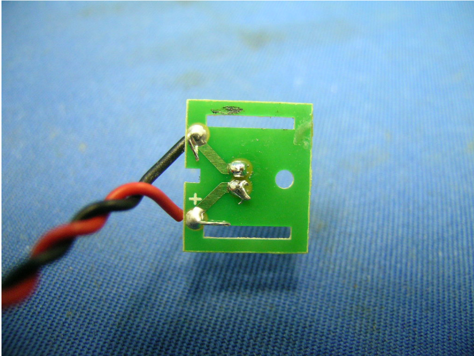
Base Unit Mic. Board rear side
