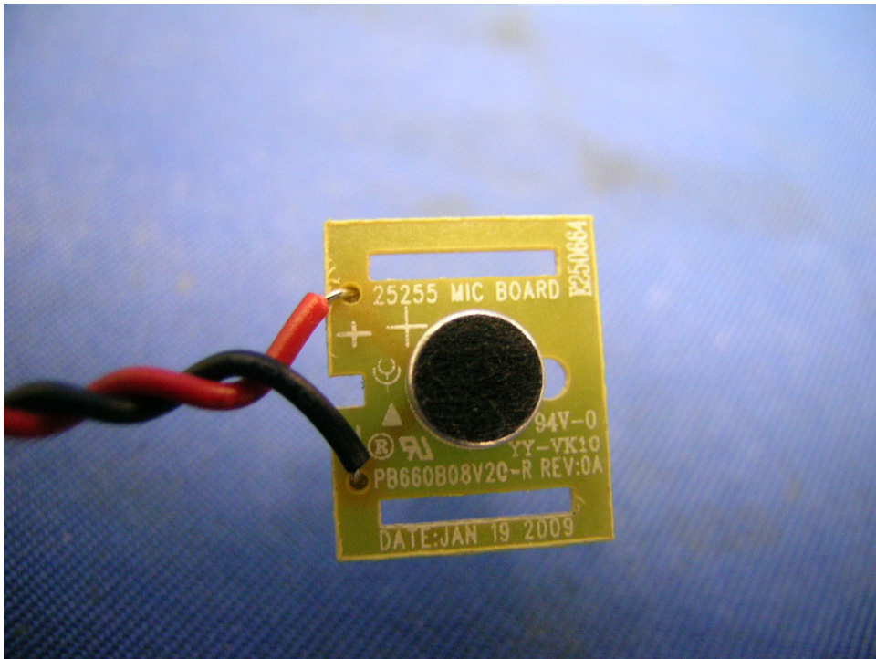
Base Unit Mic. Board front side
